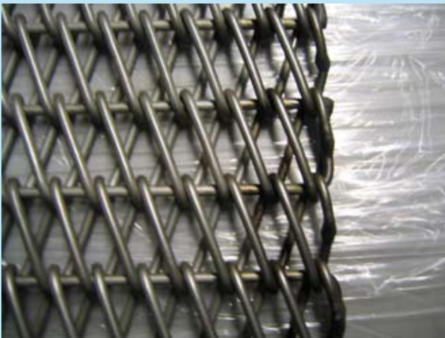
Treillis double tiges
